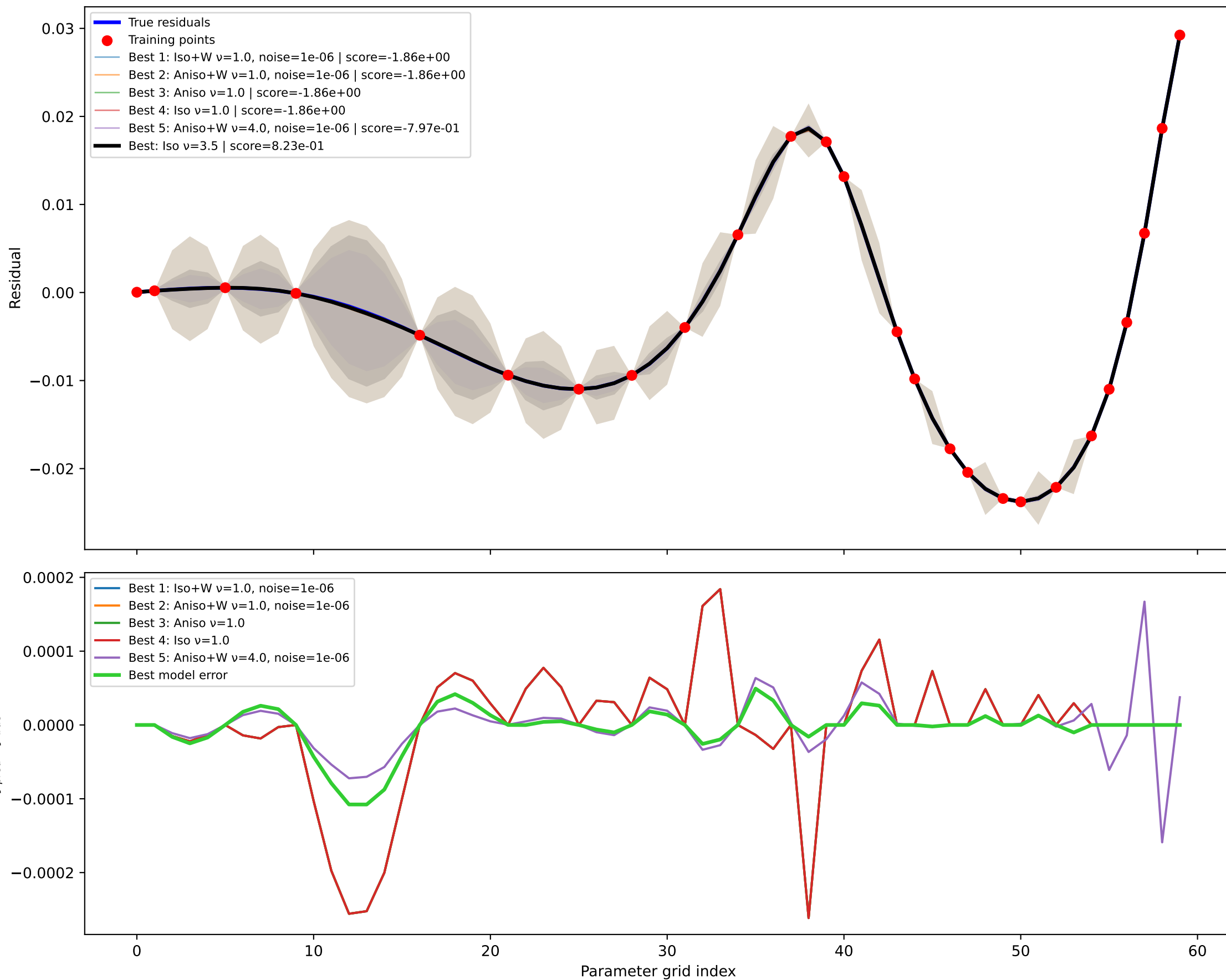
GPR kernel comparison node=14 RMSE=3.018e-05, train RMSE=1.068e-10
